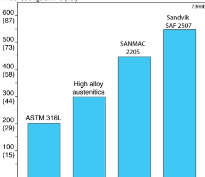
Figure 1. Comparison of proof strengths, 0.2% offset, of Sanmac SAF 2205, high alloy austenitic grades and other grades, for material in the solution annealed and quenched condition.
