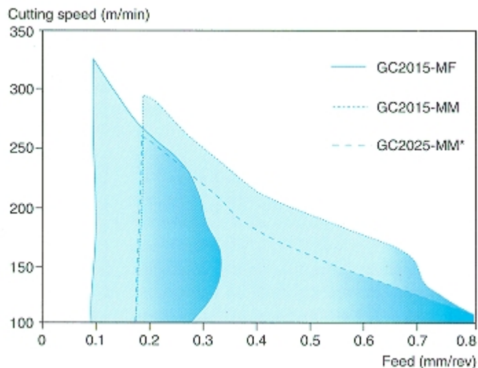
Figure 1. Machining chart for Sanmac 304/304L.
