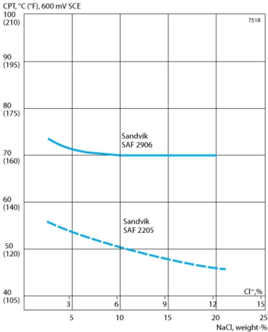
Figure 3. Critical pitting temperature (CPT) at varying concentrations of sodium chloride, from 3 to 25%
