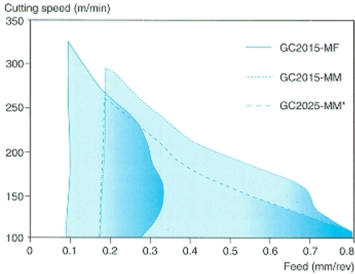
Figure 1. Machining chart for Sanmac 4435.
