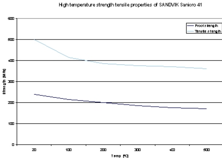
Figure 1. Minimum high temperature tensile strength properties for Sanicro 41 are based on datasheets seamless tube and pipe. Since the tubes have thin walls the values should only be used as indicative values for forgings. (Proof strength corresponds to 0.2% offset yield strength.)
