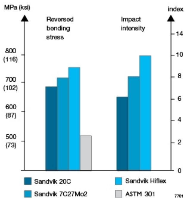
Figure 1. Comparison of fatigue properties for Sandvik's flapper valve steels and a standard spring steel (ASTM 301)
