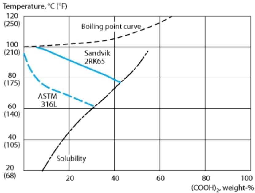
Figure 4. Isocorrosion diagram 0.1 mm/year (4mpy) for 2RK65 and ASTM 316L in oxalic acid.
