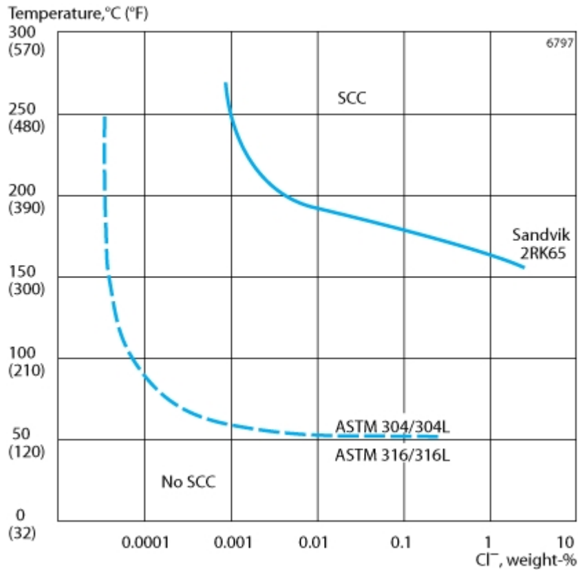
Figure 10. SCC resistance of 2RK65 in comparison to ASTM 304 and AISI 316 types of steels in neutral aerated chloride environments.
