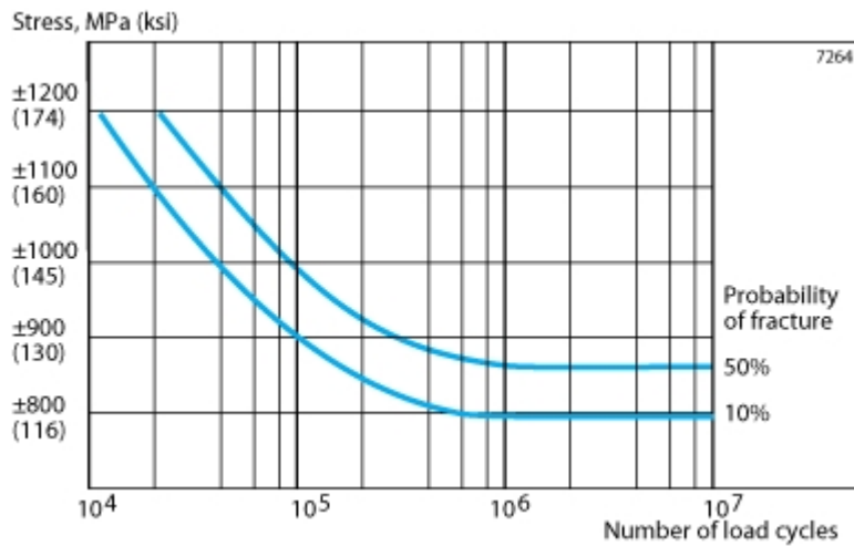
Figure 2. Wöhler S-N curve for Sandvik 7C27Mo2, tensile strength 1800 MPa (261000 psi), max. thickness 1.00 mm (0.0394 in.). Thicker materials have a somewhat lower fatigue strength. The diagram shows that Sandvik 7C27Mo2 with a maximum thickness of 1.00 mm (0.0394 in.) has a fatigue limit of 860 MPa (125000 psi).
