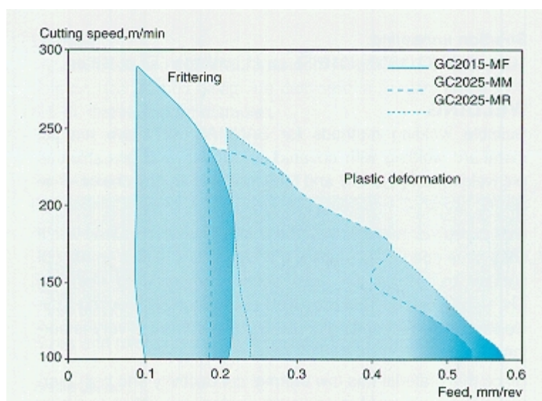
Figure 1. Machining chart for Sanmac 4541.
