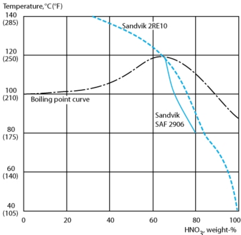
Figure 6. Iso- corrosion diagram for SAF 2906™ and Sandvik 2RE10 in a naturally aerated, stagnant solution of nitric acid. The curves represent a corrosion rate of 0.1 mm/year.
